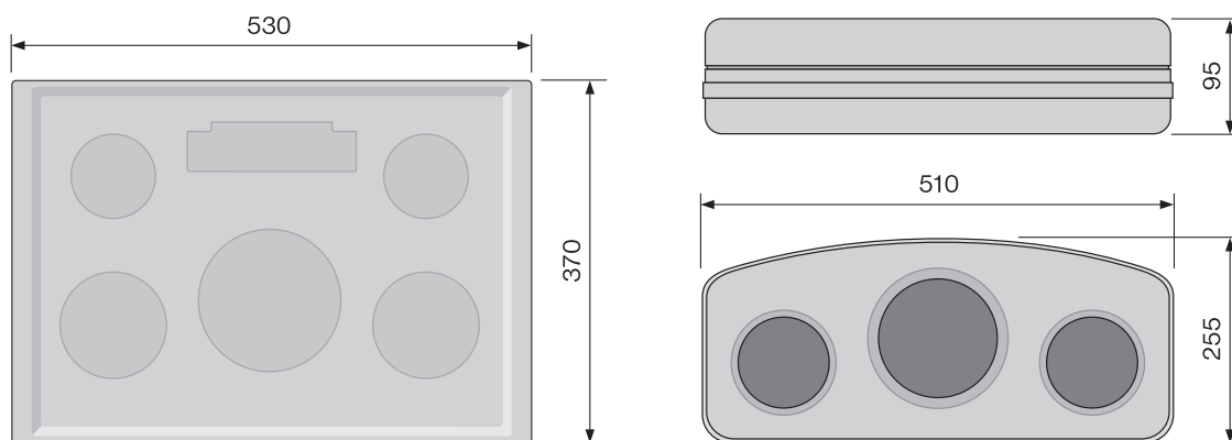
29001 Tray THERMOLINE 530×370
